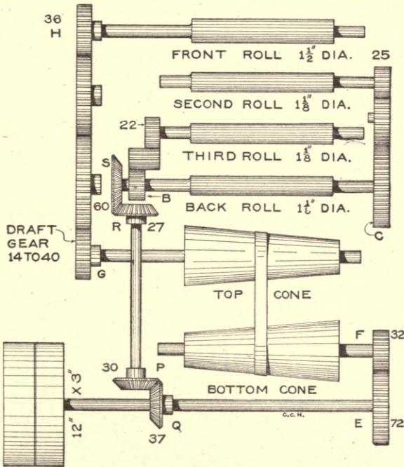
Fig. 138. Diagram of Railway Head Draft Gearing.
